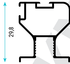
TD-974 0,314 Kg/m Dar Kulp / Narrow Handle Profile
