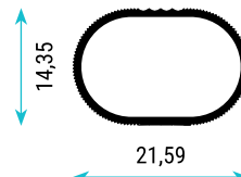
TD-980 0,150 Kg/m Oval Askı
