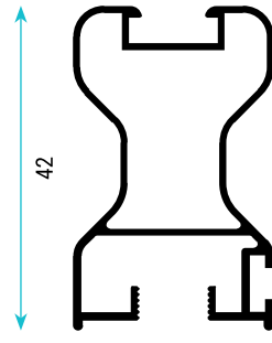
TD-1333 0,440 Kg/m Geniş Kulp / Wide Handle Profile
