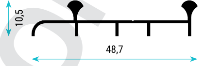
TD-977 0,233 Kg/m Erkek Alt Ray / Beta Lower Rail Profile
