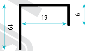
TD-3828 0,127 Kg/m Topal 18mm U
