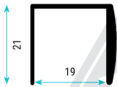
TD-1359 0,243 Kg/m 18mm Oval Yanak U
